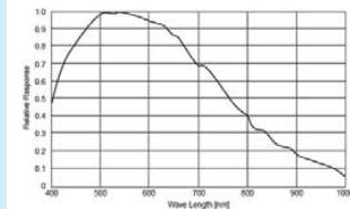
Spectral Sensitivity for G0433B
