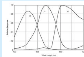
Spectral Sensitivity for G0433C
